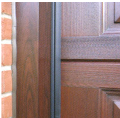
Neat all round rubber weather seal. Note how door is mounted onto back of standard 3" timber frame.
